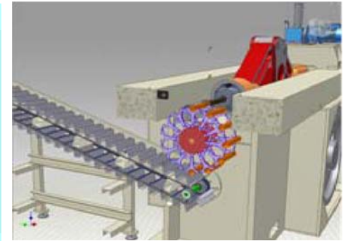
Can take-off unit
