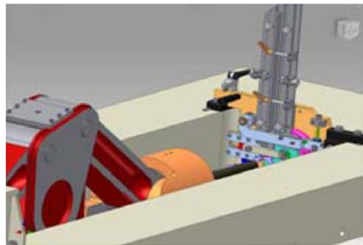
Hydraulic quick tool clamping system to reduce set up time
