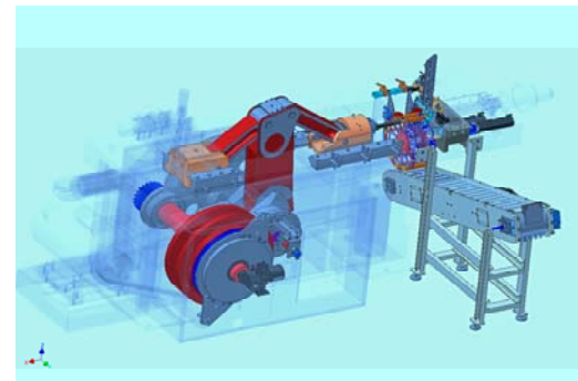
Loading and unloading system
