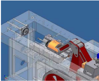
Double knuckle-joint: 30% impact speed reduction
